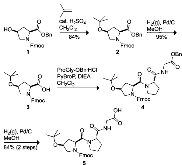
Scheme 1. Synthesis of Fmoc-hyp( t Bu)ProGly-OH (5)
