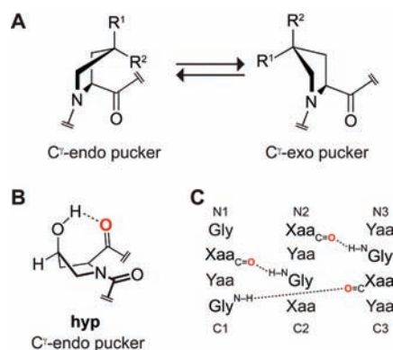
Figure 1. Attributes of Pro derivatives. (A) The pucker of the pyrrolidine ring can be enforced by the gauche effect arising from an electronegative C \gamma substituent (R 1 or R 2 ), which adopts the pseudoaxial position. Hyp: R 1 = OH, R 2 = H; hyp: R 1 = H, R 2 = OH; Mop: R 1 = OMe, R 2 = H; mop: R 1 = H, R 2 = OMe. (B) Intramolecular hydrogen bond in hyp. (C) Interstrand hydrogen bonds in a collagen triple helix. O i of a hyp residue in the Xaa position is red in panels B and C.
