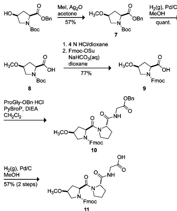
Scheme 2. Synthesis of Fmoc-mopProGly-OH (11)
