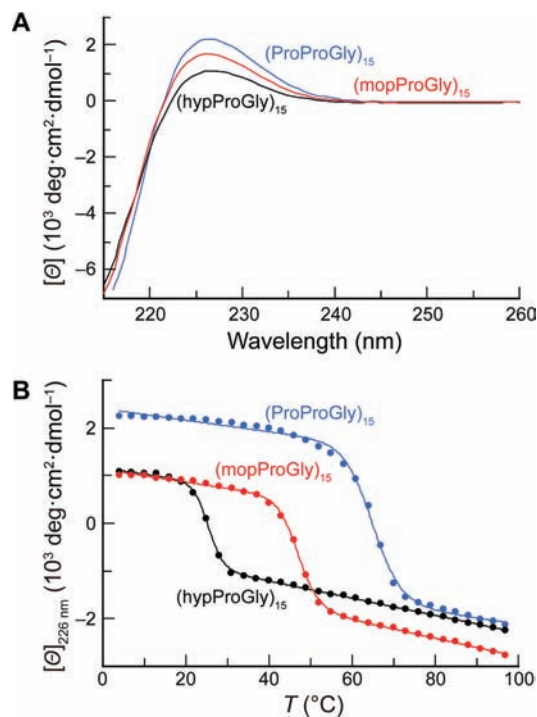
Figure 4. Conformational analysis of (hypProGly) 15 , (mopProGly) 15 , and (ProProGly) 15 by CD spectroscopy. (A) Spectra of peptide solutions (0.2 mM in 50 mM acetic acid) incubated at \leq 4 °C for \geq 24 h. (B) Effect of temperature on the molar ellipticity at 226 nm. Data were recorded at intervals of 3 °C after equilibration for \geq 5 min.
