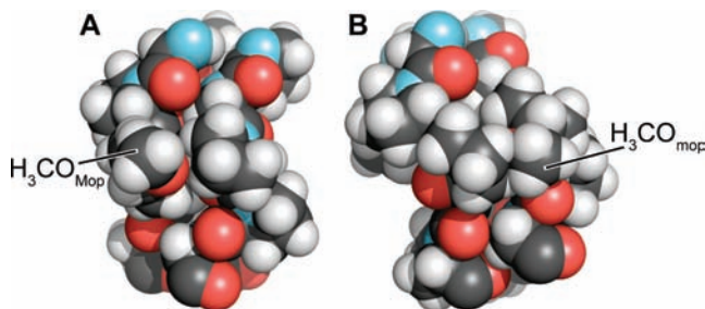
Figure 6. Space-filling models of a segment of a (\text{ProMopGly})_n and (\text{mopProGly})_n triple helix. Models were constructed from the three-dimensional structure of a (\text{ProProGly})_n triple helix (PDB entry 1k6f 10 ) by replacing the appropriate hydrogen with a methoxy group in its least hindered conformation using the program SYBYL (Tripos, St. Louis, MO). Models were depicted with the program PyMOL.
