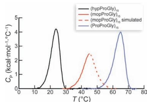
Figure 5. DSC scans of (hypProGly) 15 (122 \mu M), (mopProGly) 15 (122 \mu M), and (ProProGly) 15 (96 \mu M) in 50 mM HOAc (pH 3.0; scan rate = 6 °C/h).
